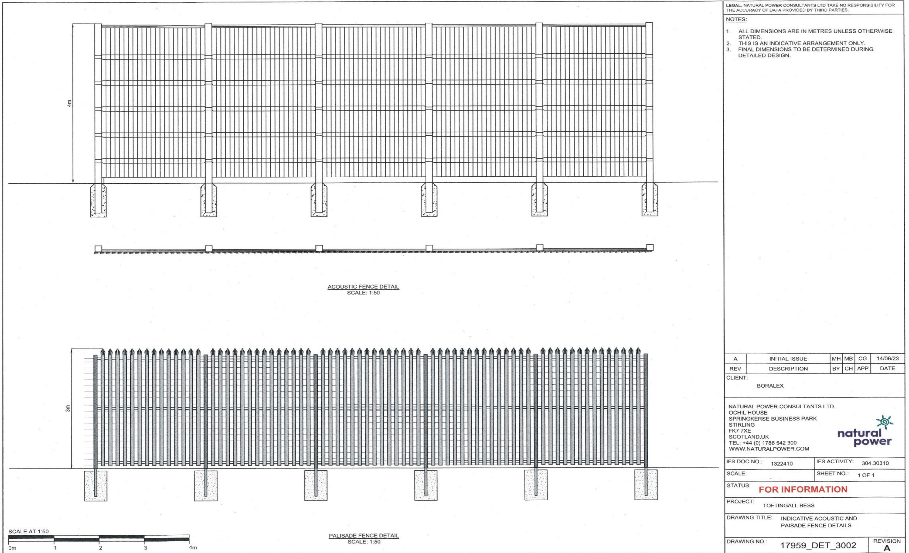
Figure 4.5: Indicative Fence Details
