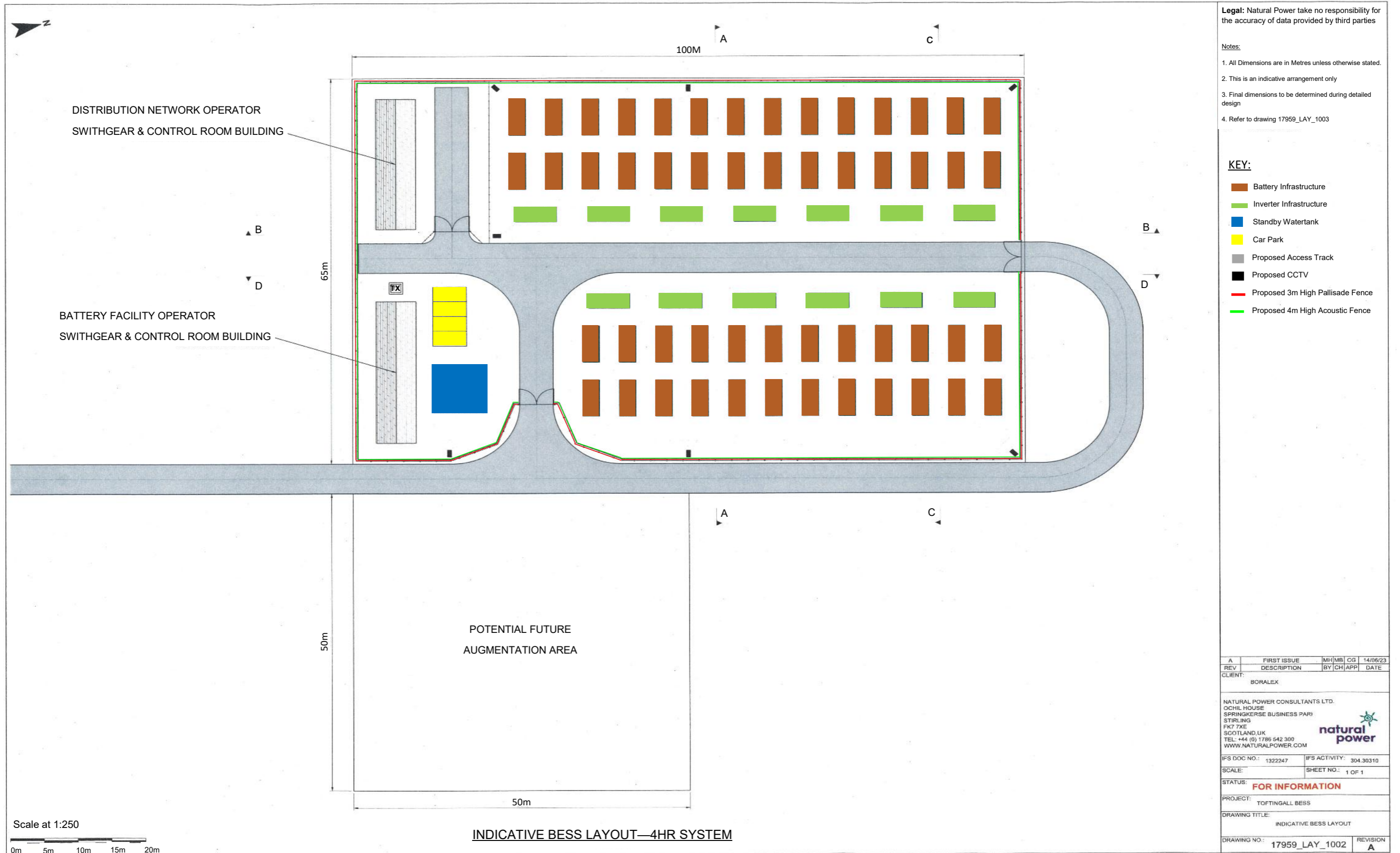
Figure 4.2: Indicative BESS Layout
