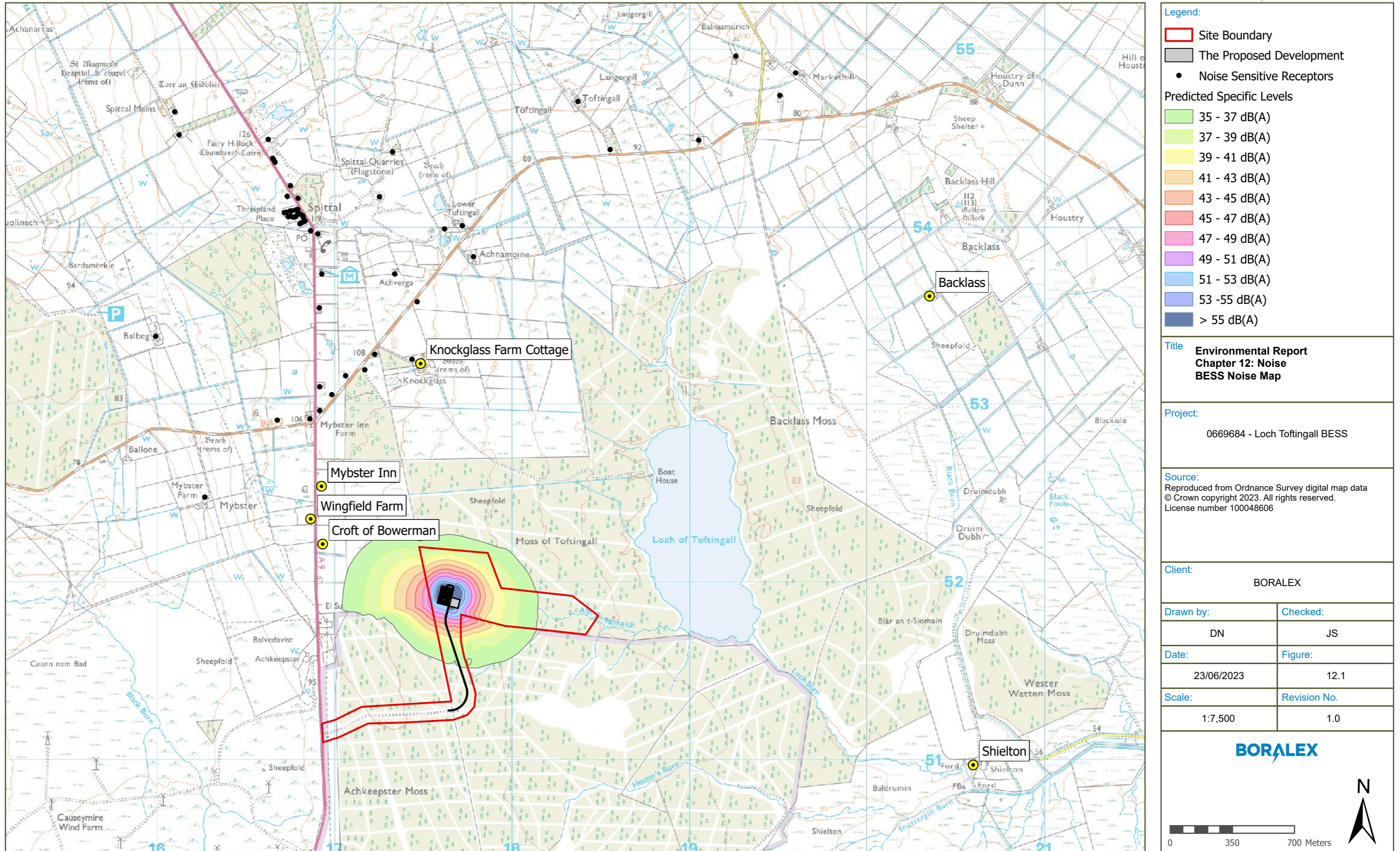
Figure 12.1: Noise Map
