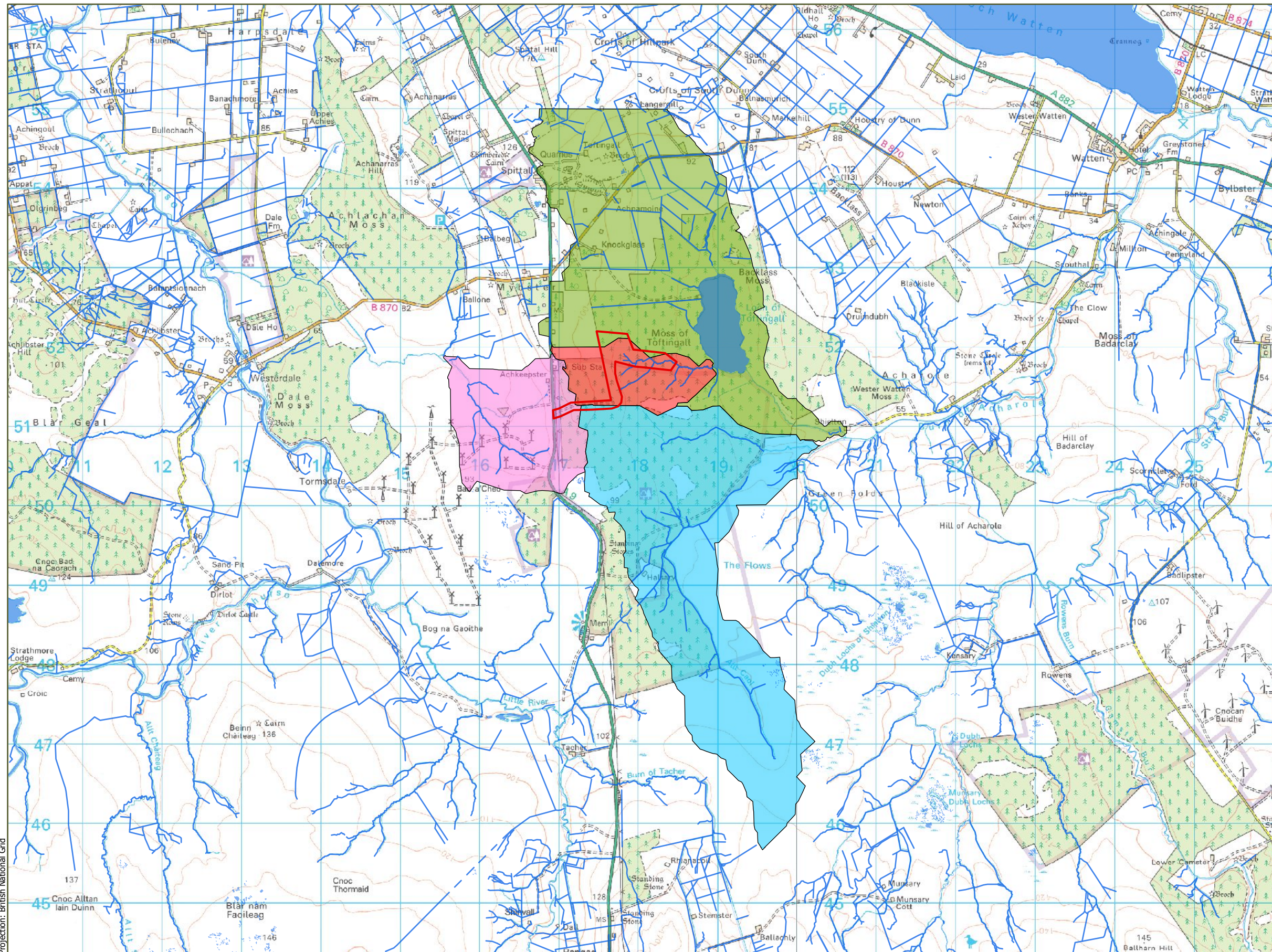
Figure 11.2: Surface Hydrology
