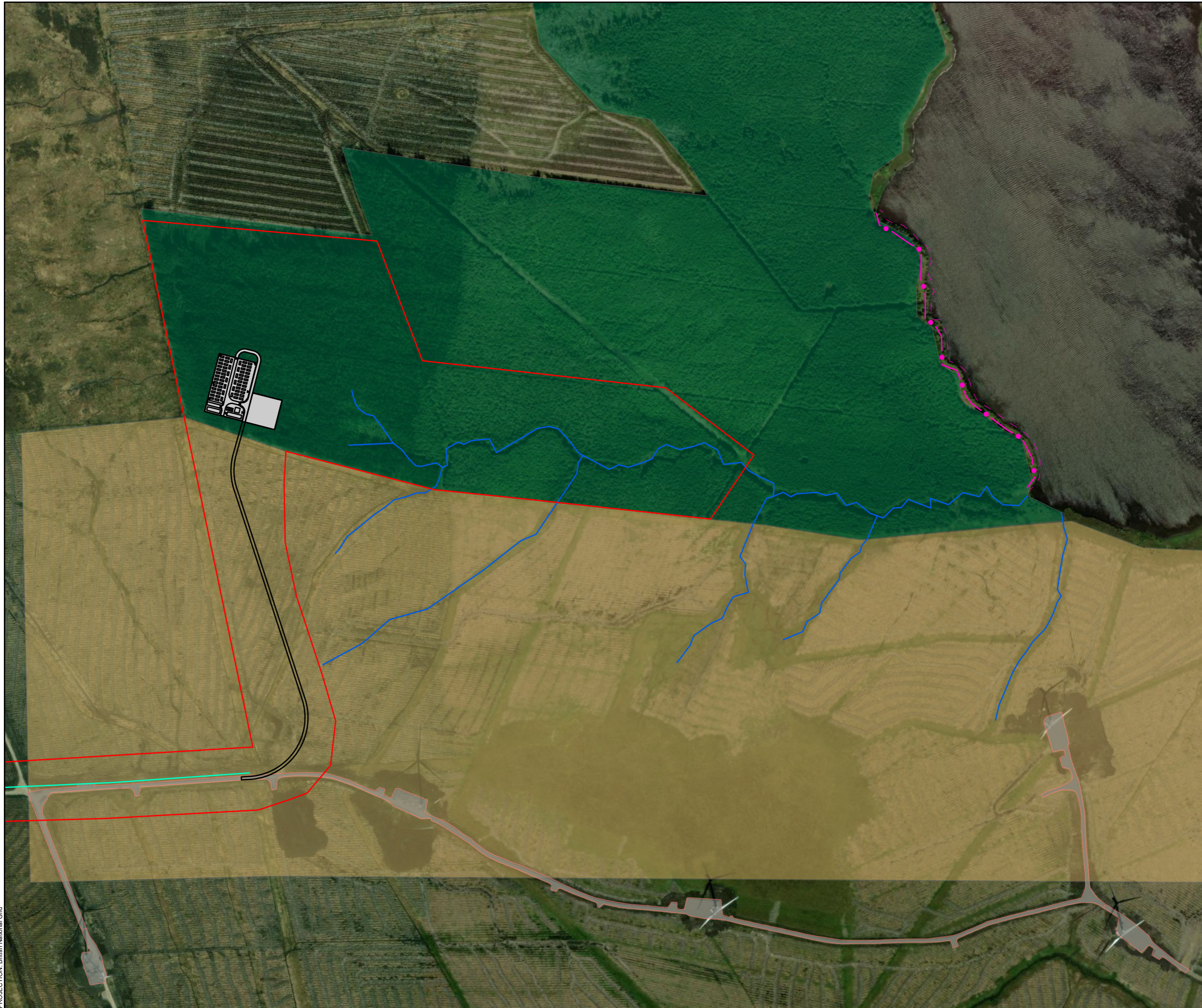
Loch Toftingall BESS - Environmental Report Technical Appendix A10.1: Peat Slide Risk Assessment Figure 10.1.4: Geomorphology Map
